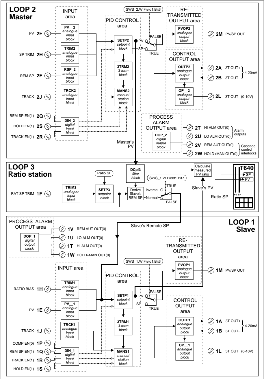
Figure 5-9 Strategy #4 schematic
