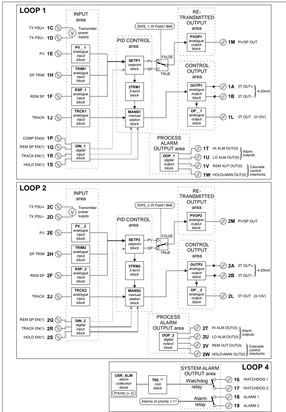
Figure 5-5 Strategy #2 schematic
