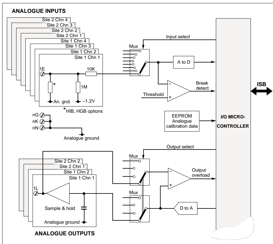
Figure 9-2 Analogue input & output block schematic
