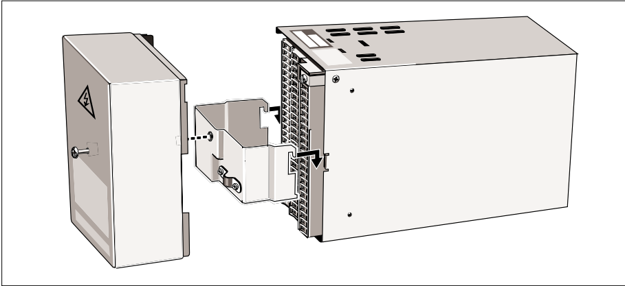
Figure 3-1 Terminal cover removal
