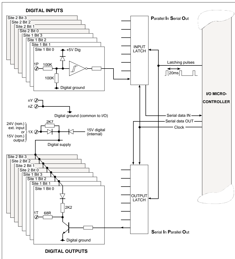
Figure 9-3 Digital input &amp; output block schematic
