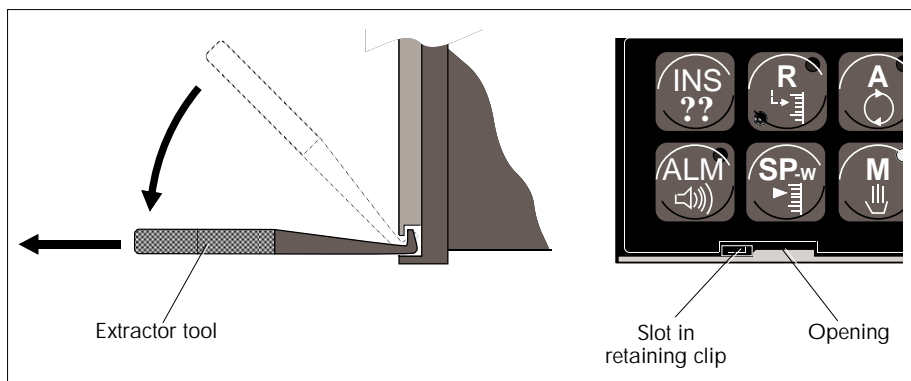
Figure 2-4 Withdrawing T640 from the sleeve
