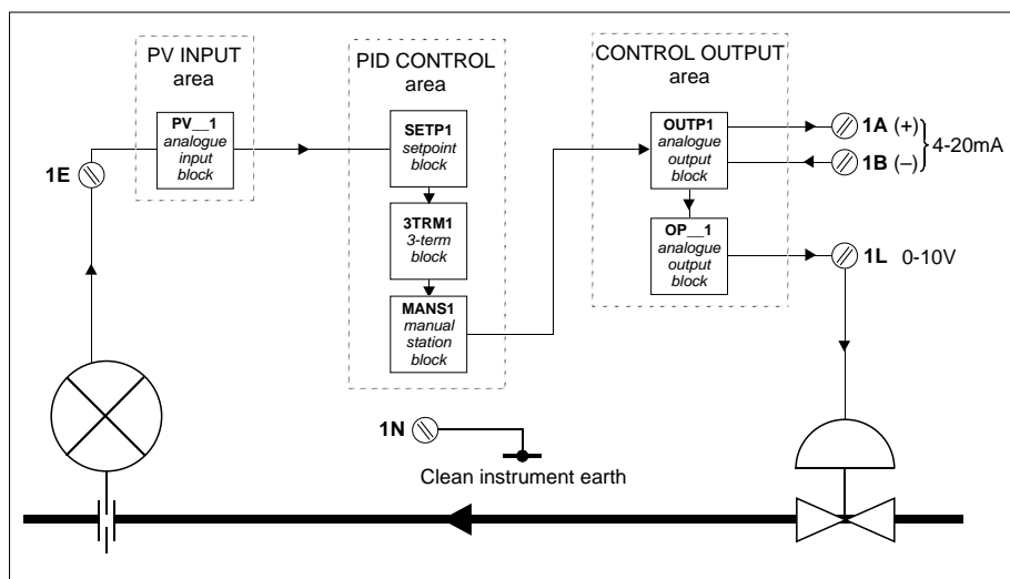
Figure 3-9 Strategy #1 schematic
