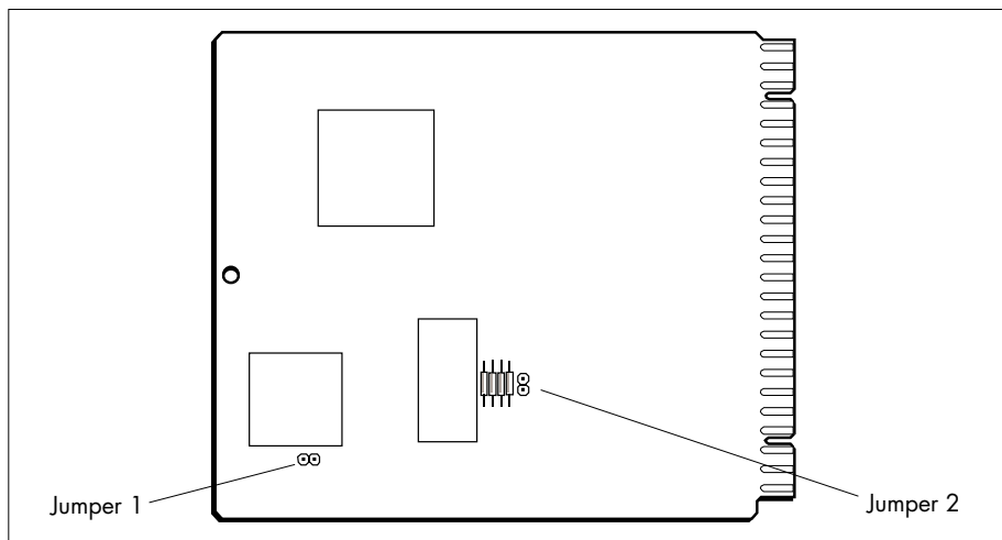
Figure 9-1 High-level I/O board showing 0 - 1.25V range jumpers
