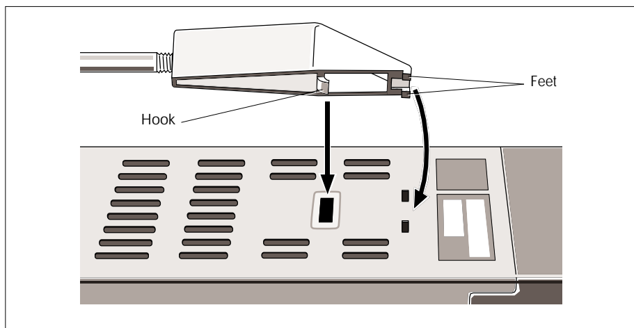
Figure 2-2 Fitting a clamp to the sleeve
