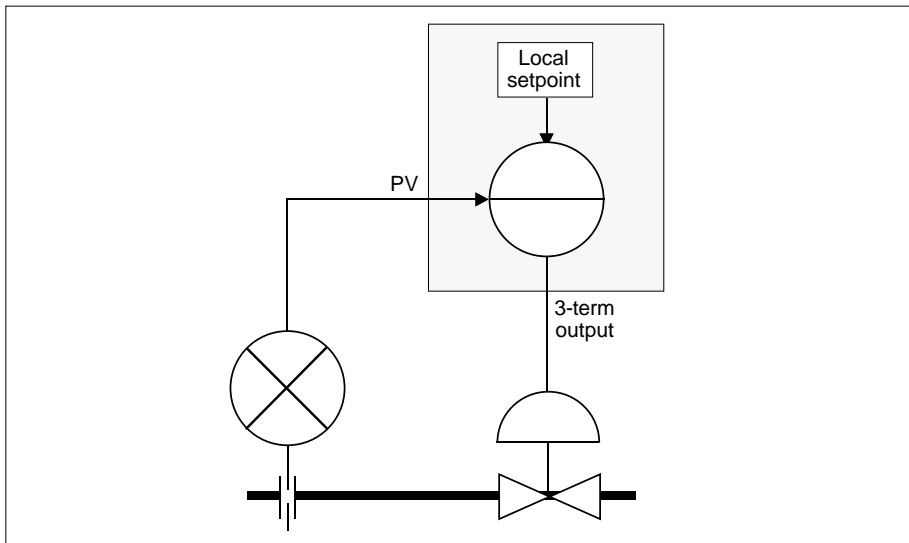
Figure 3-5 Example P &amp; I diagram for strategy #1
