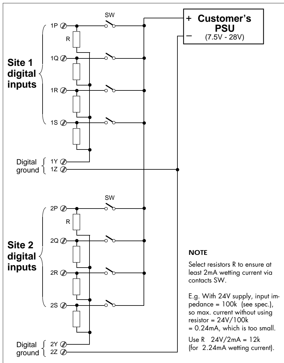
Figure 9-7 Digital input contact-sensing using customer's PSU
