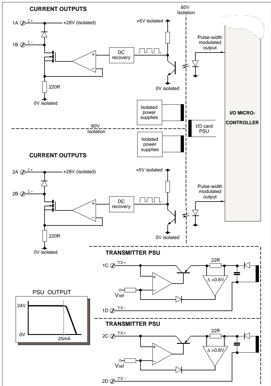
Figure 9-4 Current output &amp; transmitter PSU block schematic
