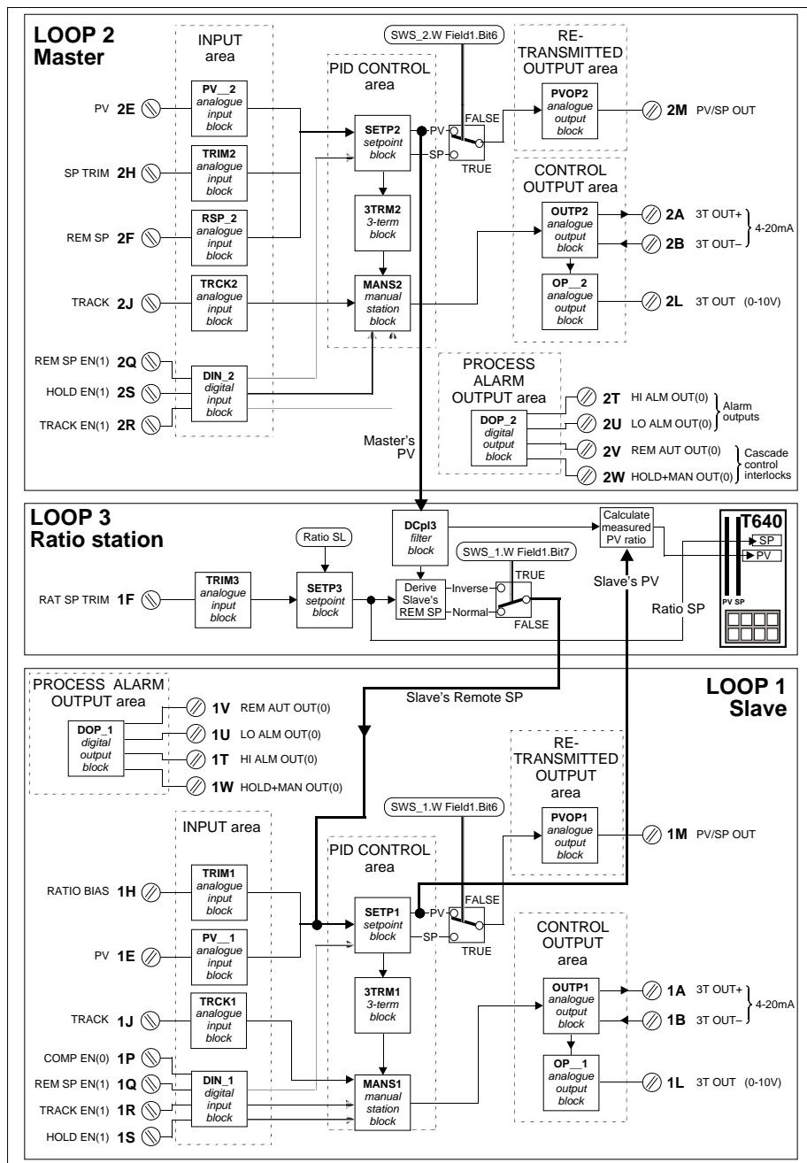
Figure 5-9 Strategy #4 schematic
