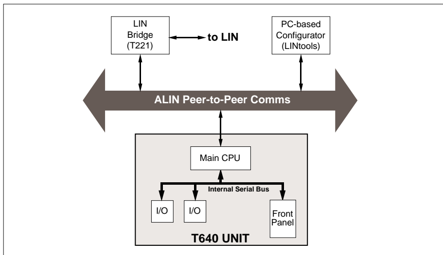
Figure 7-2 ALIN communications schematic
