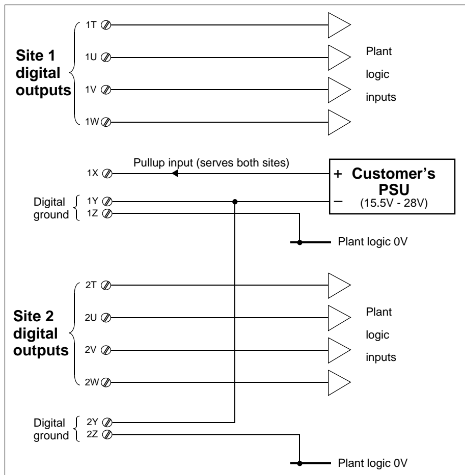
Figure 9-5 Digital outputs driving plant logic using customer's PSU
