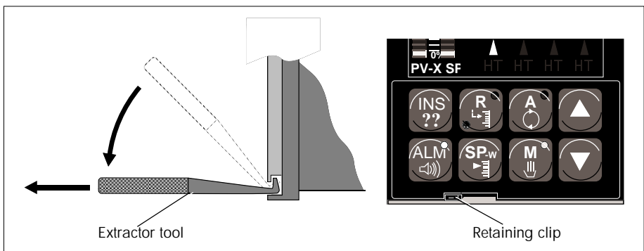
Figure 3-3 Removal of T640 from sleeve
