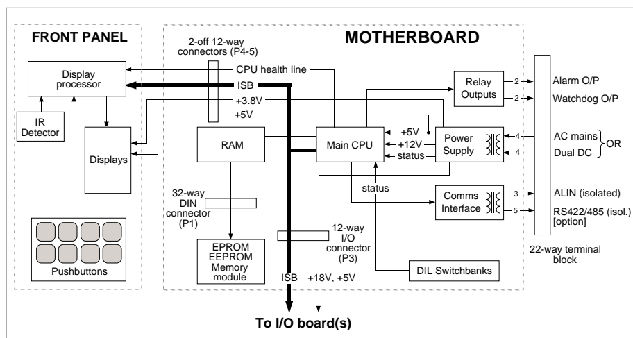
Figure 7-1 T640 Functional block schematic
